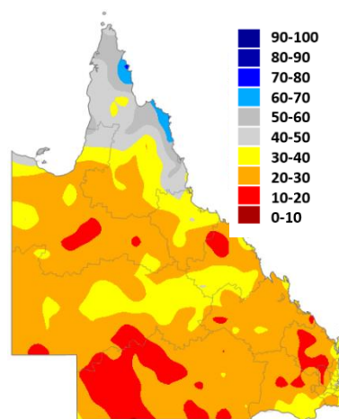
Fig. 11: Probability of exceeding median rainfall for July to September 2026 based on a 'Consistently Negative' phase of the SOI at the end of June 2026.
