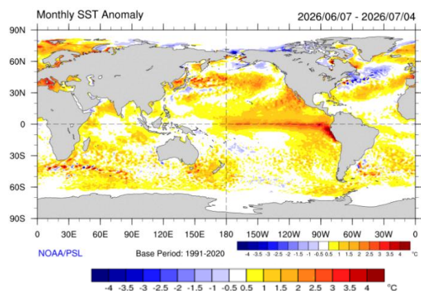
Fig. 6: Pacific Ocean sea-surface temperature anomalies (°C) for to 7 June to 4 July 2026 based on NOAA OISST.v3.1 SST data (1991 to 2020 based period) Map source: https://psl.noaa.gov/map/clim/sst.shtml
