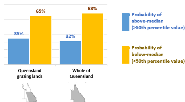
Fig. 9: Probabilities of above and below median summer rainfall (for November to March) as at 1 July 2026.
