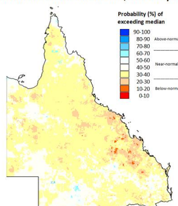
Fig. 8: Probability of exceeding median summer rainfall (for November 2026 to March 2027) as at 1 July 2026
