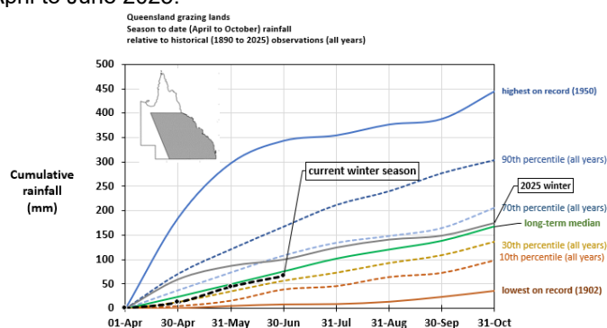
Fig. 4: April to October 2026 season accumulated rainfall as at 1 July 2026, compared to historical values.
