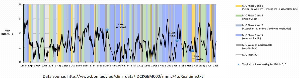
Fig. 7: Madden-Julian Oscillation intensity and phase-location
