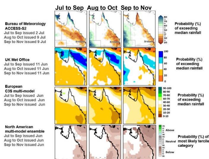
Fig. 10: Rainfall probabilities for July to Nov 2026, based on international dynamical models.
