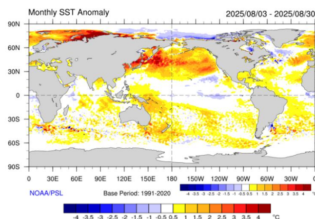
Fig. 6: Pacific Ocean sea-surface temperature anomalies (°C) for 3 to 30 August 2025 based on NOAA OISST.v3.1 SST data (1991 to 2020 based period) Map source: https://psl.noaa.gov/map/clim/sst.shtml
