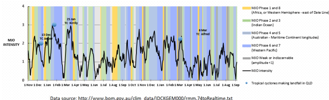
Fig. 7: Madden-Julian Oscillation intensity and phase-location
