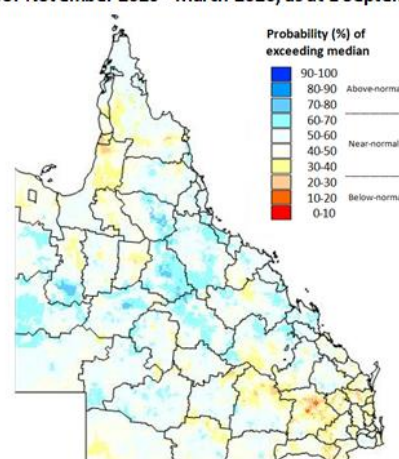
Fig. 8: Probability of exceeding median summer rainfall (for November 2025 to March 2026) as at 1 September 2025 Produced by the DETSI SPOTA-1 system.
