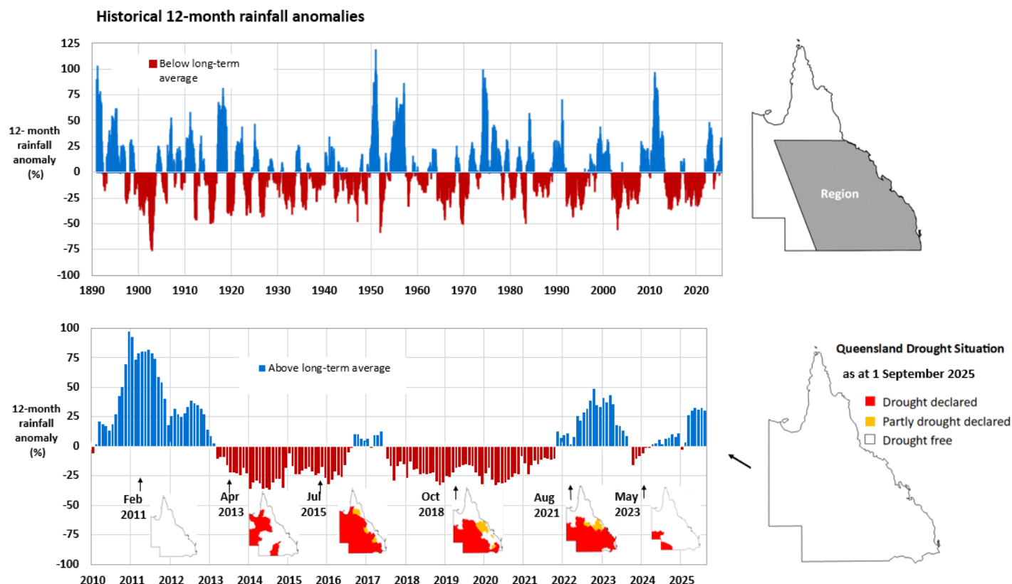
Fig.1: Historical 12-month rainfall anomalies
