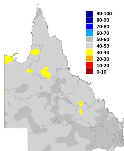
Fig. 11: Probability of exceeding median rainfall for September to November 2025 based on a 'Consistently Near Zero' phase of the SOI at the end of August 2025.
