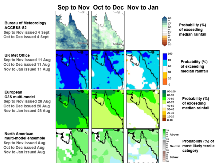
Fig. 10: Rainfall probabilities for September 2025 to January 2026, based on international dynamical models.
