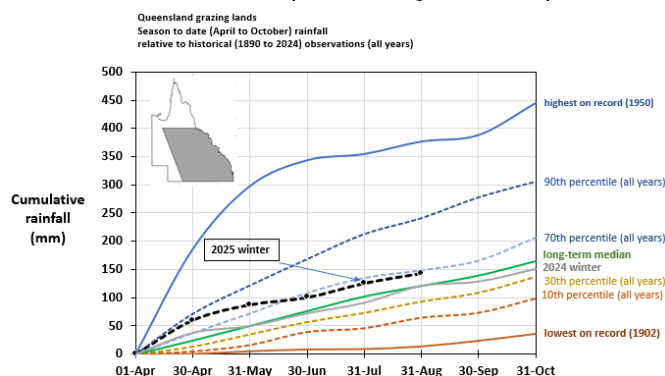
Fig. 4: April to October 2025 season accumulated rainfall as at 1 September 2025, compared to historical values.
