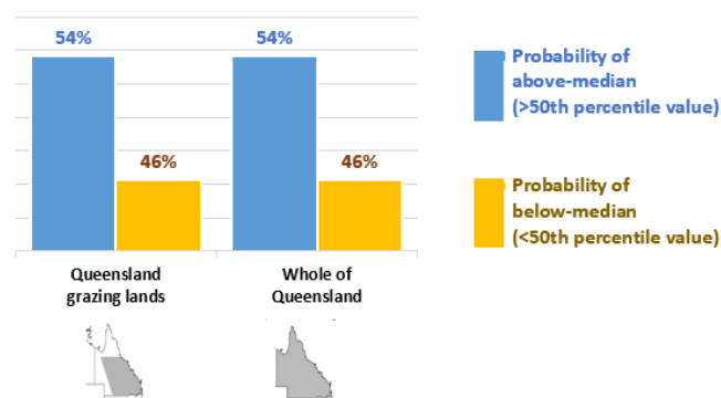
Fig. 9: Probabilities of above and below median summer rainfall (for November to March) as at 1 September 2025.
