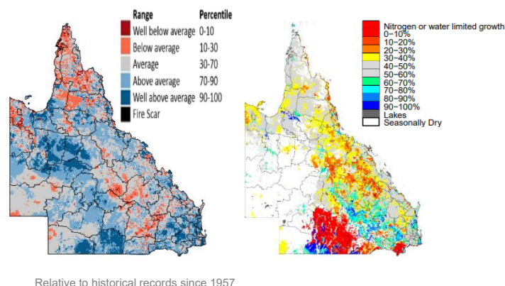
Fig. 12: Calculated pasture cover at 31 August 2025.
