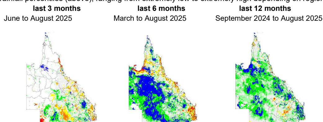
Fig. 3: Pasture growth percentiles (base period 1957 to current)
